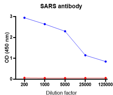
Figure 1: Specificity of anti-SARS (MQR2.3901), determined by ELISA. Antibody stock 1.38 mg/ml diluted in PBS containing 0.05% tween-20 and 1% BSA was tested on human Seryl-tRNA-synthetase (in blue) and non-target protein (in red)..
