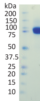
Figure 1. NuPage analysis of purified PDGF-R \beta -ECD
